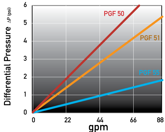
Clean ΔP of PROGAF™ Filter Bags (Water at ambient conditions)
