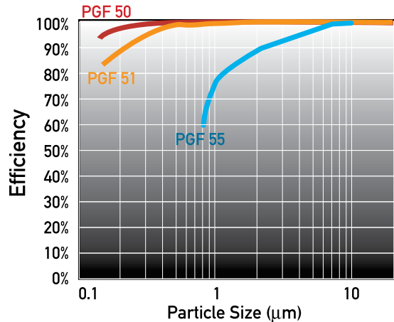
Fractional Efficiency of PROGAF™ Filter Bags (ISO Fine in water at ambient conditions @ 90 gpm)
